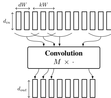
Figure 2: Illustration of a convolutional layer. d_{in} and d_{out} are the dimension of the input and output frames. kW is the kernel width (here kW = 3 ) and dW is the shift between two linear applications (here, dW = 2 ).
